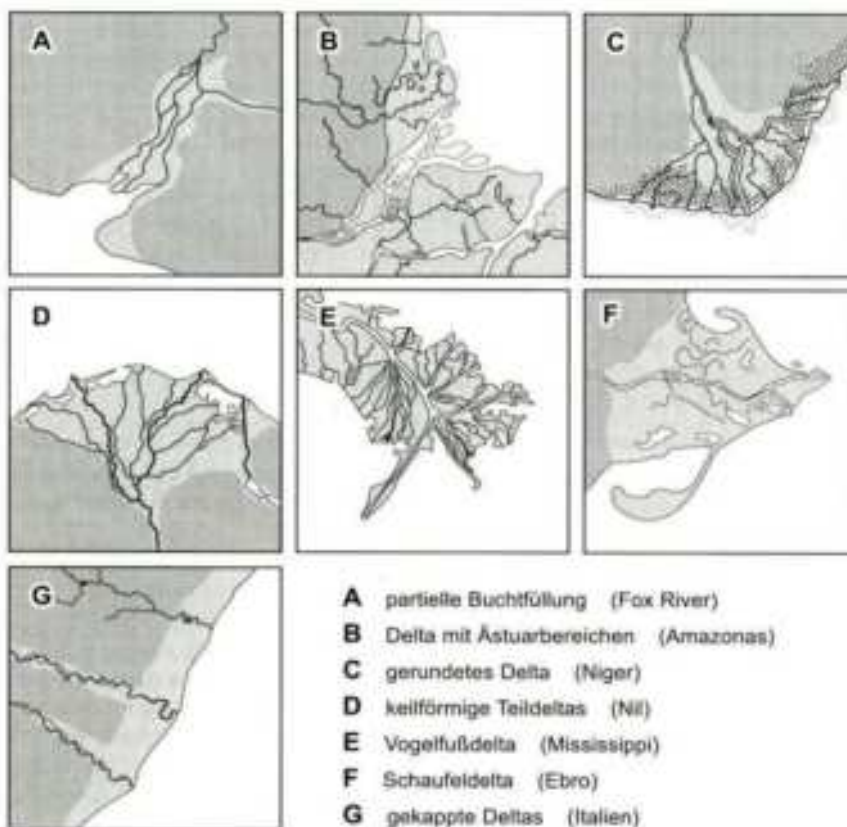
Figure 1: Types of deltas (from Ahnert 2001). The most common Mediterranean delta types are those shown in D, F and G. The Mediterranean deltas are generally river-sediment-driven and not predominantly wave-formed or tidal.
