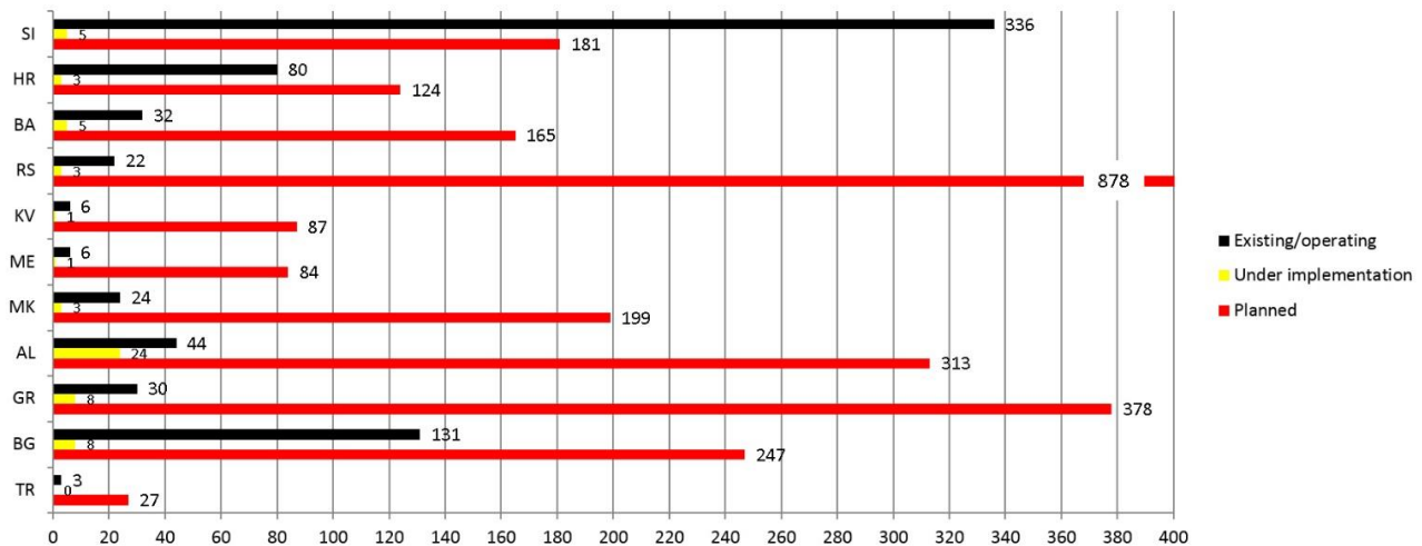
Figure 2: Country distribution of hydropower plants for entire Balkan region
